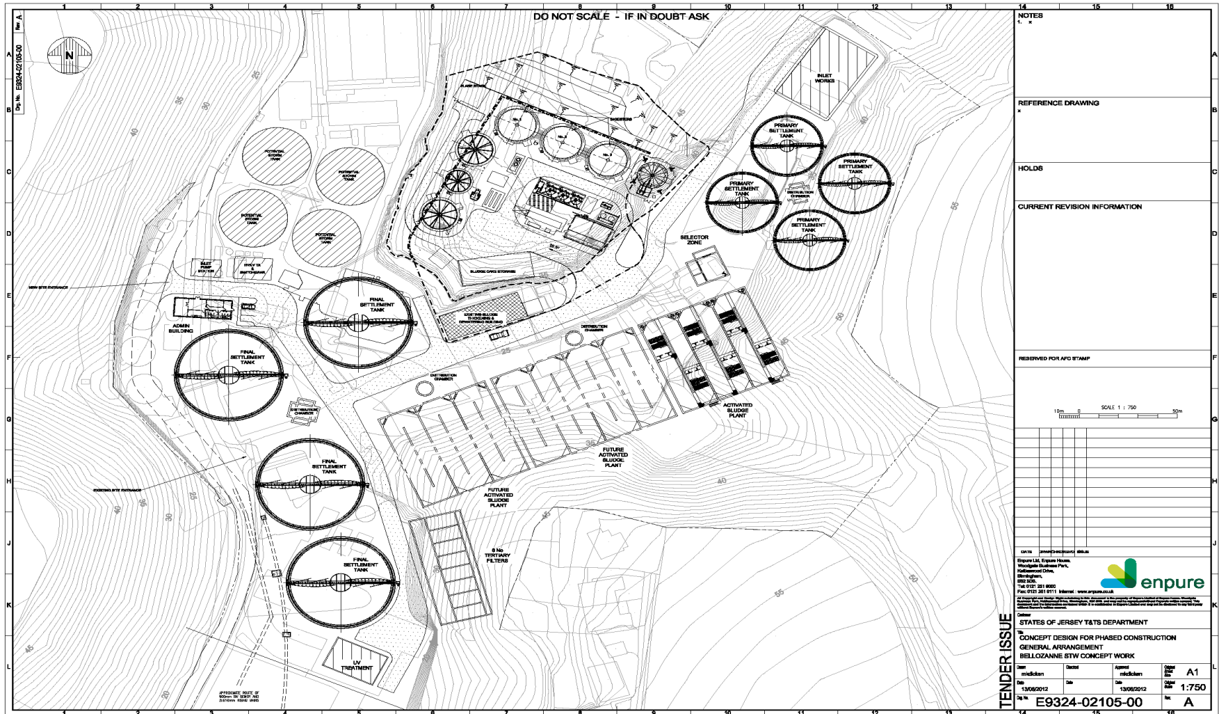
Figure 1: Proposed Phased Construction For Bellozanne STW
